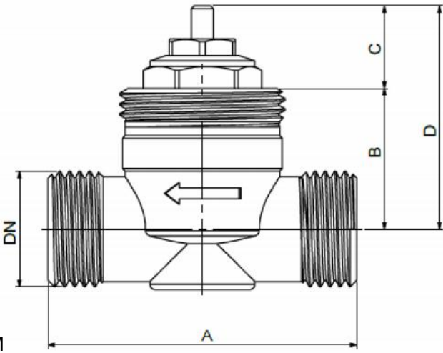
尺寸图： Dimensional drawing
